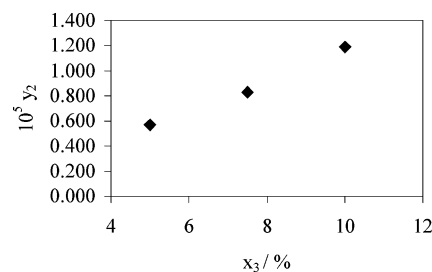
Figure 4. Effect of cosolvent, at 15.0 MPa and 313.0 K, as a function of x_3 .
