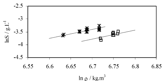
Figure 6. Logarithmic relationship between the solubility of acetazolamide and the density of the mixture (CO 2 + ethanol): □, 313 K; *, 323 K. The lines represent the regression fit using the Chrastil equation.
