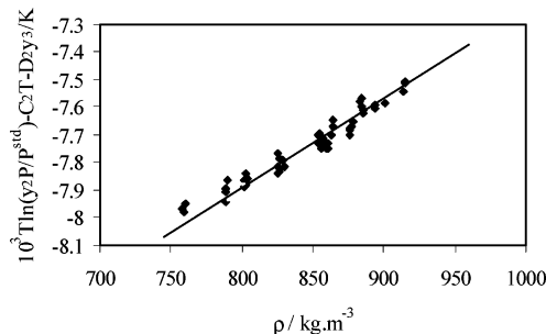
Figure 8. T \ln(y_2 p / p^{\text{std}}) - C_2 T - D_2 x_3 vs \rho : experimental solubility data correlated with eq 5.
