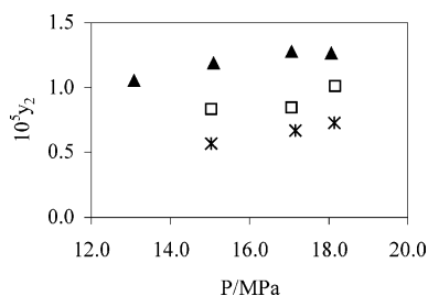
Figure 3. Mole fraction solubility of acetazolamide as a function of pressure in supercritical \text{CO}_2 in the presence of ethanol at 313 K: *, 5% ethanol; □, 7.5% ethanol; ▲, 10% ethanol.
