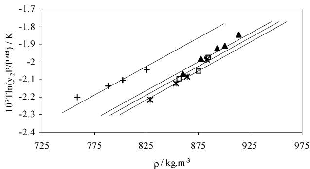
Figure 7. T \ln(y_2 p / p^{\text{std}}) as a function of \rho at 313 K: *, 5% ethanol; □, 7.5% ethanol; ▲, 10% ethanol. At 323 K, +, 5% ethanol: experimental solubility data correlated with eq 5.
