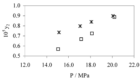
Figure 5. Effect of temperature on the solubility of acetazolamide for a mole fraction of ethanol of 5%: □, 313 K; *, 323 K.
